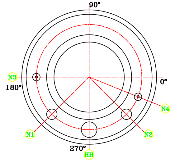
NOZZLE ORIENTATION
